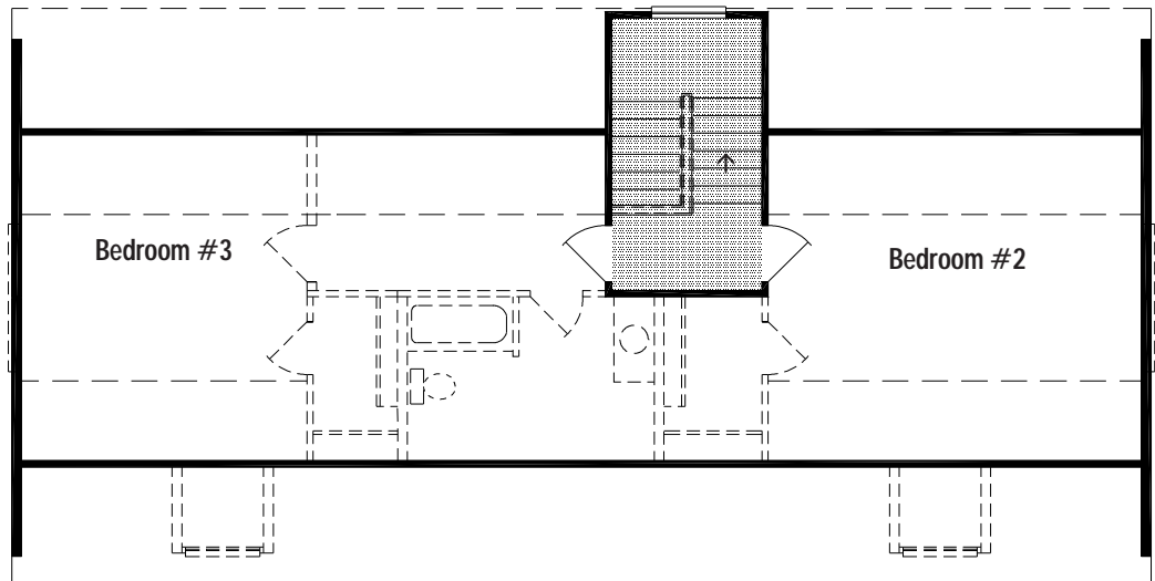
Layout A Rear Stairs (Gable Dormer) Second Floor Living Area 840 Sq. Ft.
