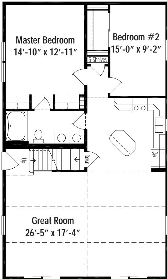
Chalet II C Basement 27'-4" x 46', First Floor Living Area 1257 Sq. Ft.
