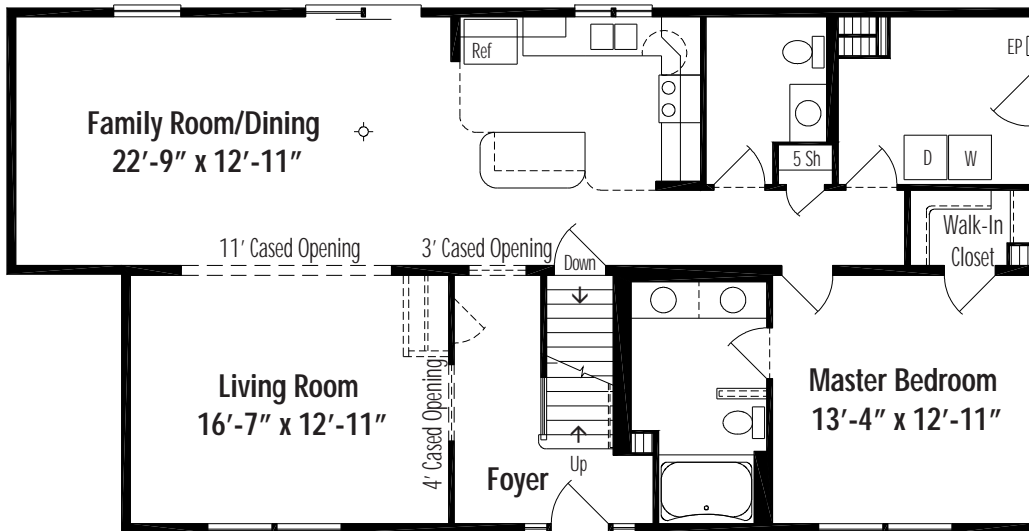
Danbury II D Basement 27'-4" x 48'/54", First Floor Living Area 1396 Sq. Ft.
