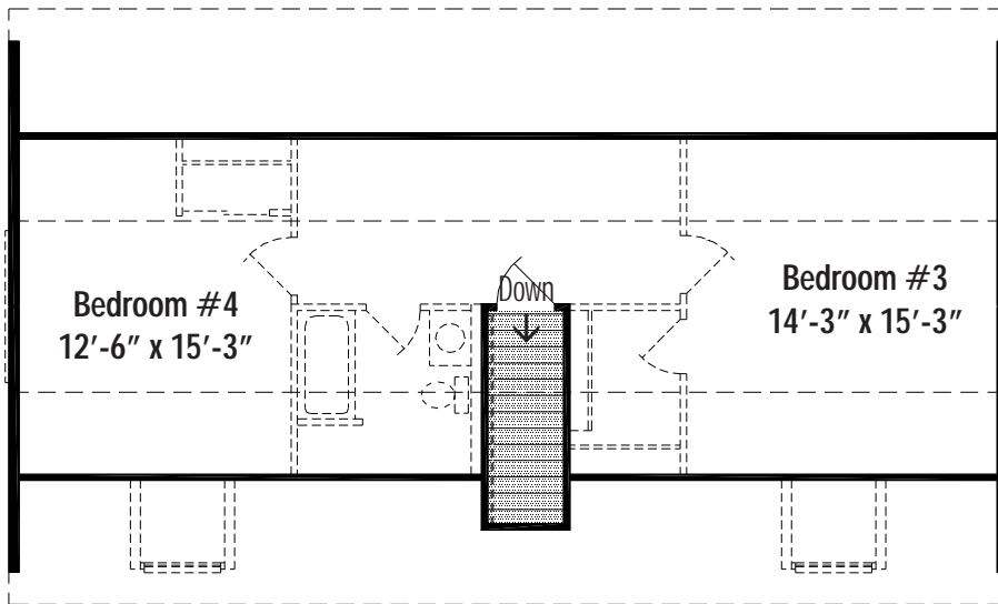
Layout A Front Stairwell Second Floor Living Area 710 Sq. Ft.
