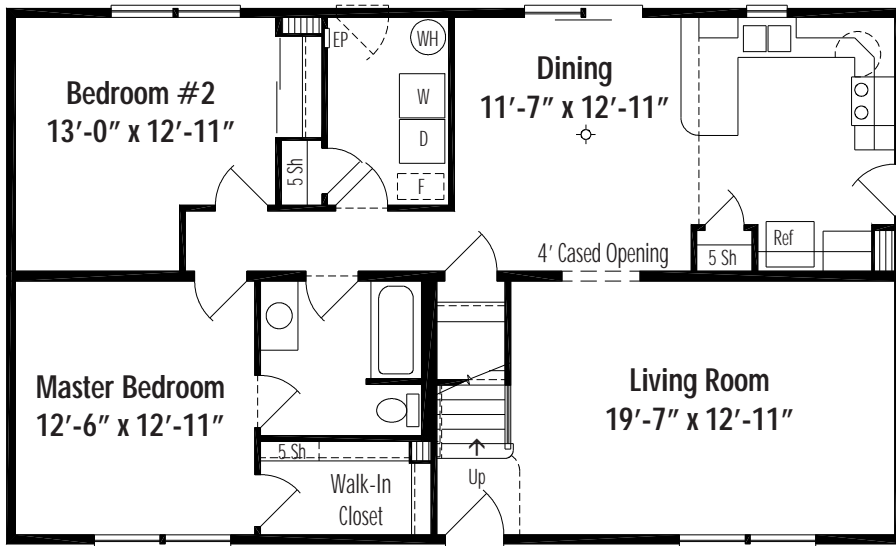
Dover C Crawl Space 27'-4" x 46', First Floor Living Area 1257 Sq. Ft.
