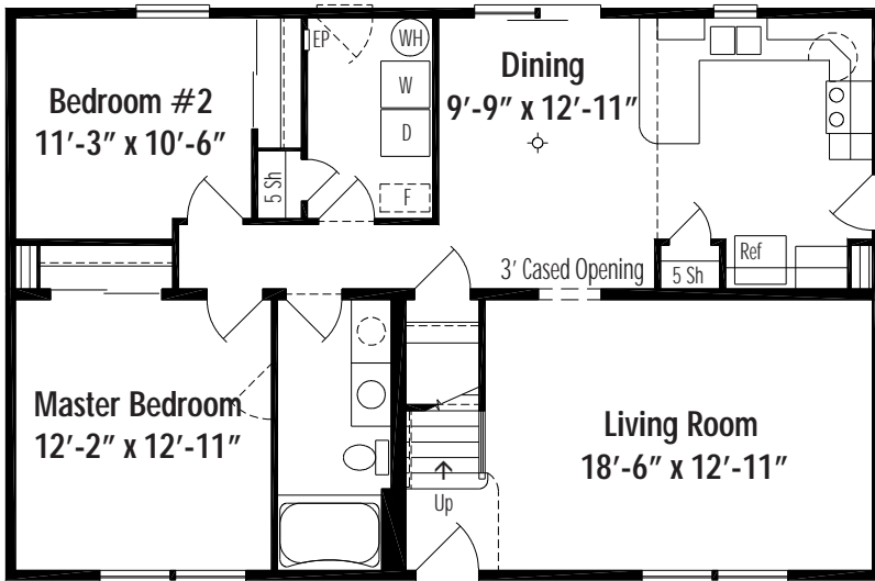
Utility Option WLU1 Alternate Utility Arrangement (Crawl Space Plan Only)
