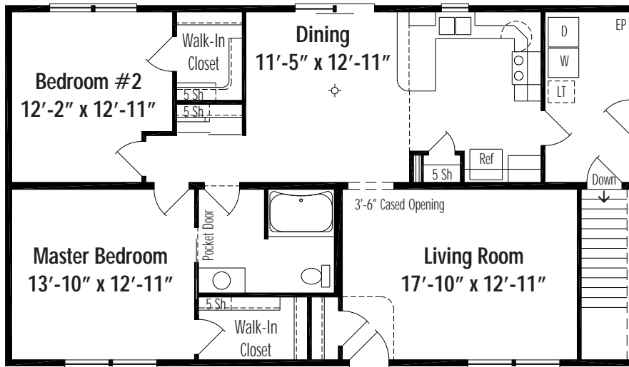
Bexley B Basement 27'-4" x 48', 1312 Sq. Ft. Living Area
