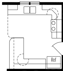
Kitchen Option D Deluxe Kitchen Available on Plans C & D
