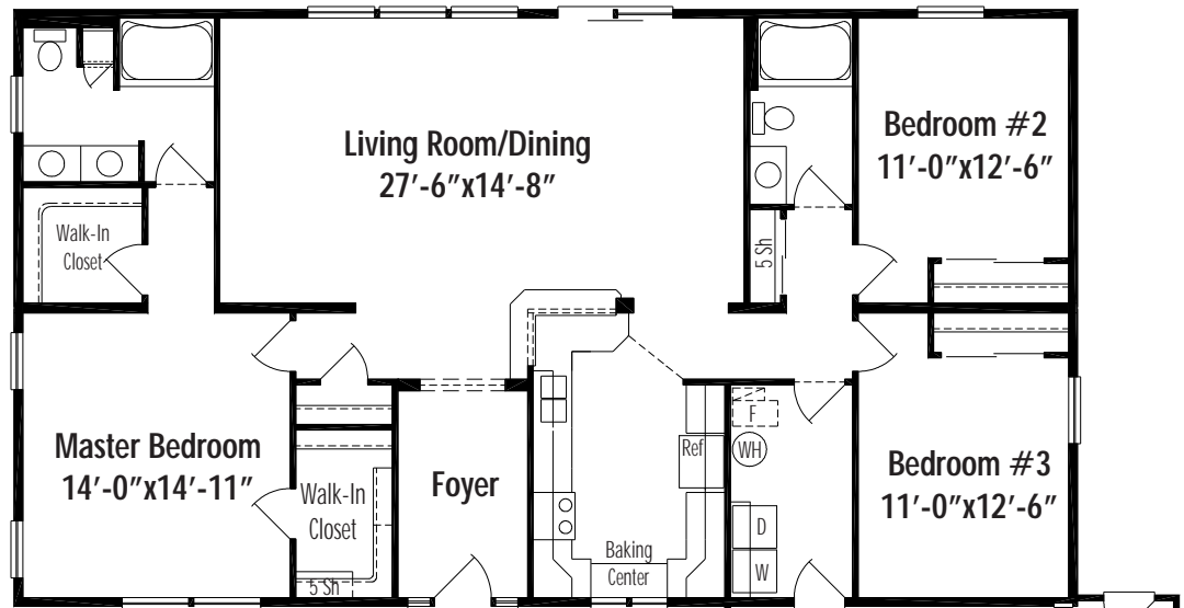
Santa Barbara A Crawl Space 31'-4" x 56', 1754 Sq. Ft. Living Area
